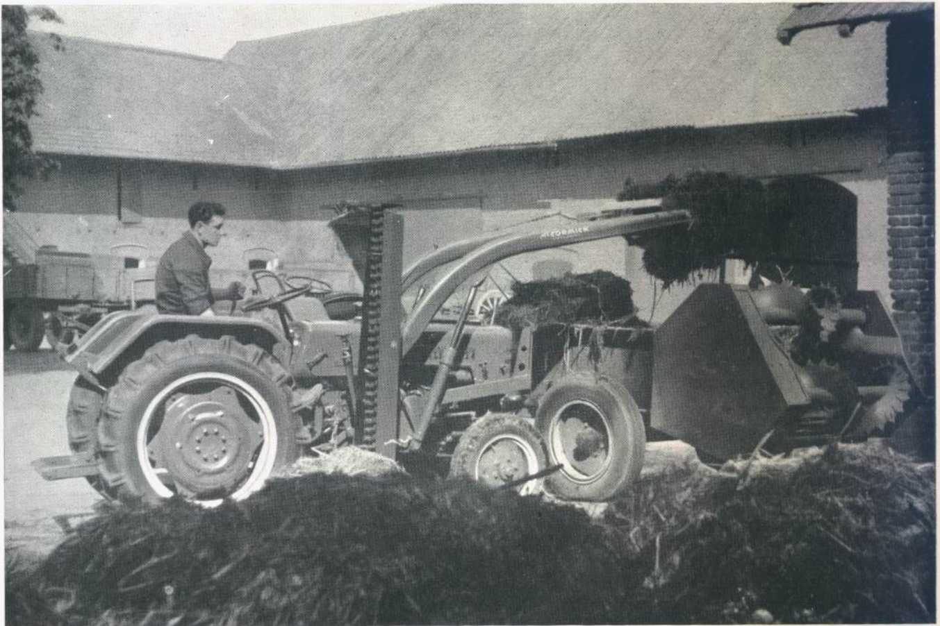
The side-mounted mower need not be removed when working with the McCormick-International Front Loader.
