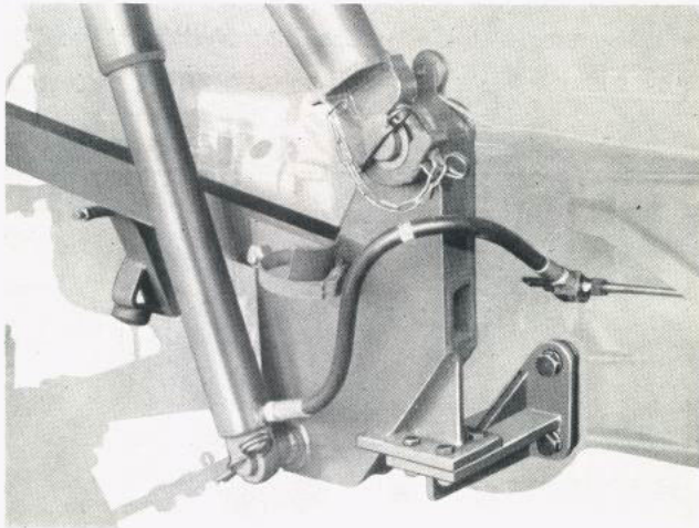
A single quick attachable mounting bracket on each side carries the boom pivot pins and hydraulic cylinder pivots.
