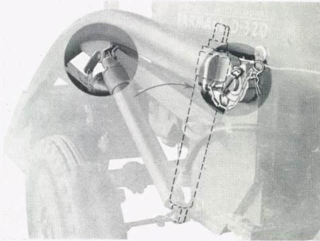
The hydraulic cylinders can be left in position, when the booms are removed, by folding the cylinders back to the position indicated above and securing them with straps.
